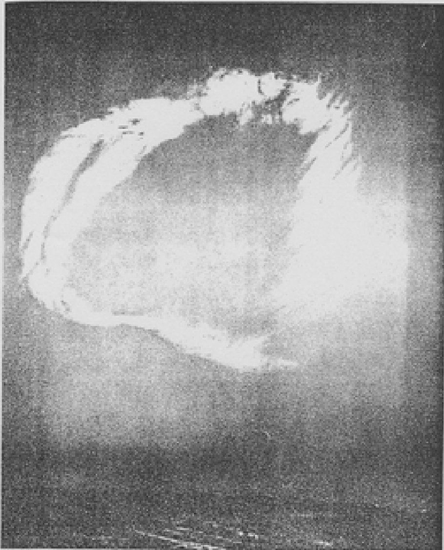
STRATOSPHERIC CLOUD
